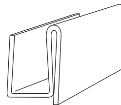
G164 — 3/8" Metal Retainer Clip G165 — 7/16" Metal Retainer Clip
